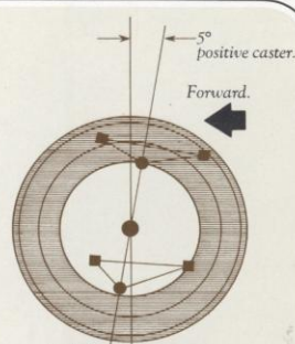
High front caster angle.
