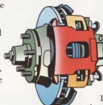
Power Disc Brakes
