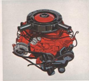
440-cu.-in. V-8 Engine. A performance-plus engine that develops 365 hp at 4600 rpm.
